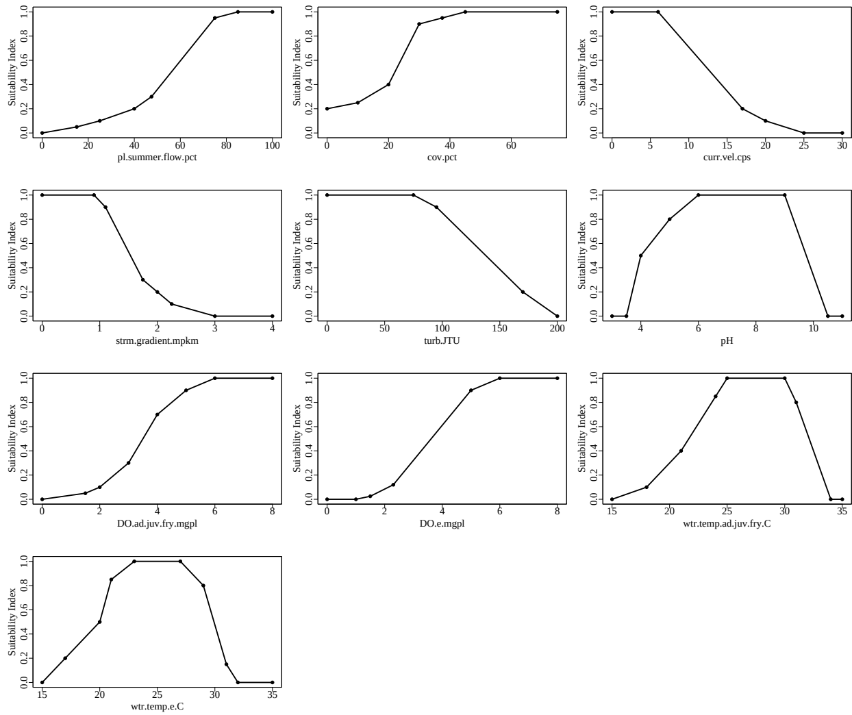
Figure 1. Suitability index graphs for variables included in the warmouthRiv model in ecorest.
